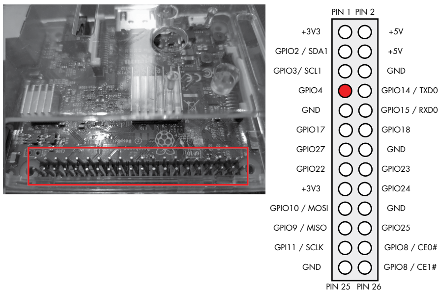
Figure 15-5: The Raspberry Pi GPIO 4 pin
