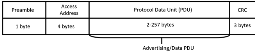
Figure 11-2: BLE's packet structure
