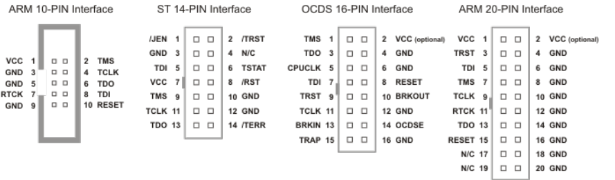
Figure 7-8: Finding any of these pin interfaces in the PCB, depending on the manufacturer (ARM, STMicroelectronics, or Infineon for OCDS), would be a good indication that you're dealing with a JTAG connector.
