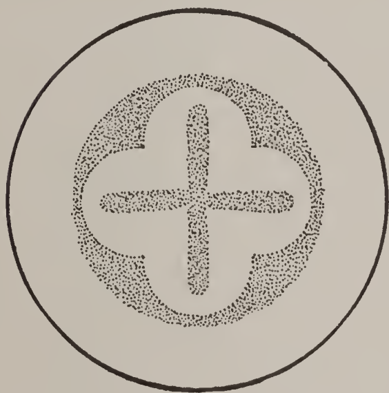
FIG. 51. — Lichtenberg's Figures.
