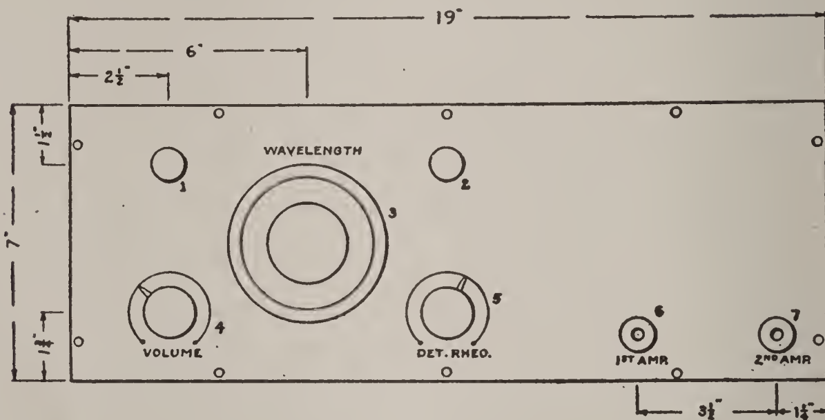
FIG. 240.—A Front View of the Panel with all the Parts in position. 1. Wavelength Switch. 2. Filament Switch. 3. Tuning Dial and Knob. 4. Volume Control Knob. 5. Detector Rheostat Knob. 6, 7. Amplifier Jacks.
