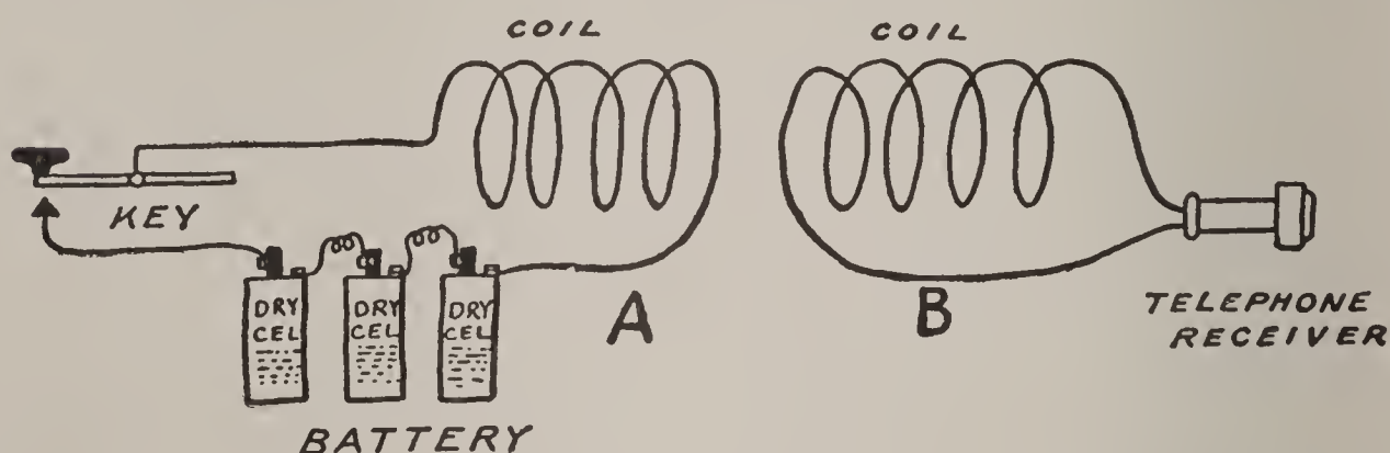
FIG. 242.—A Simple Arrangement showing the Inductive Action between two Coils.
