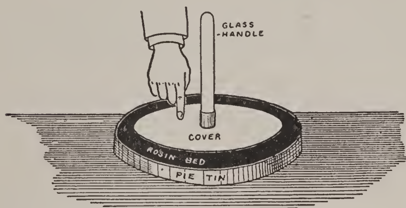
FIG. 27. — The Electrophorus.
