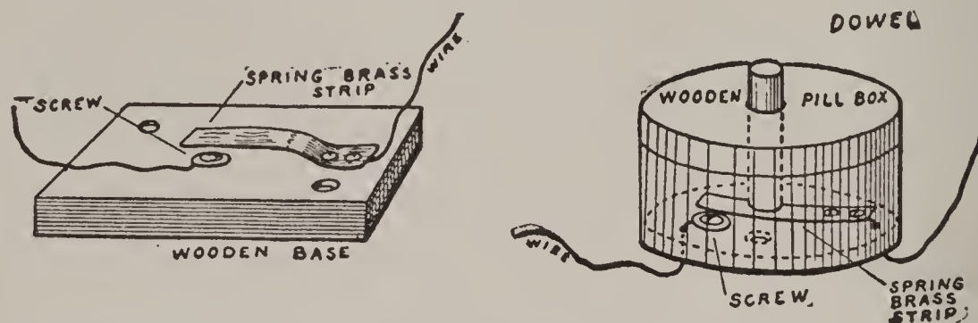
FIG. 123. — Two Simple Push-Buttons.
