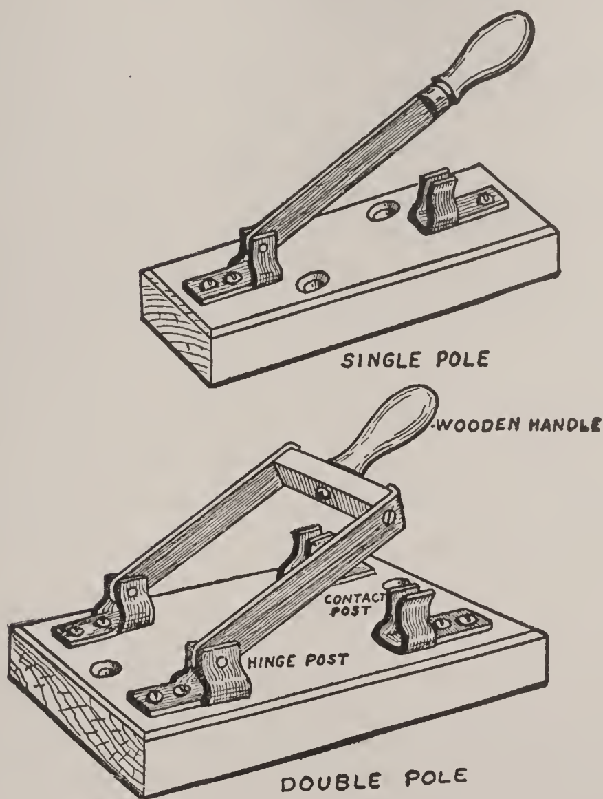
FIG. 96. — Knife Switches.
