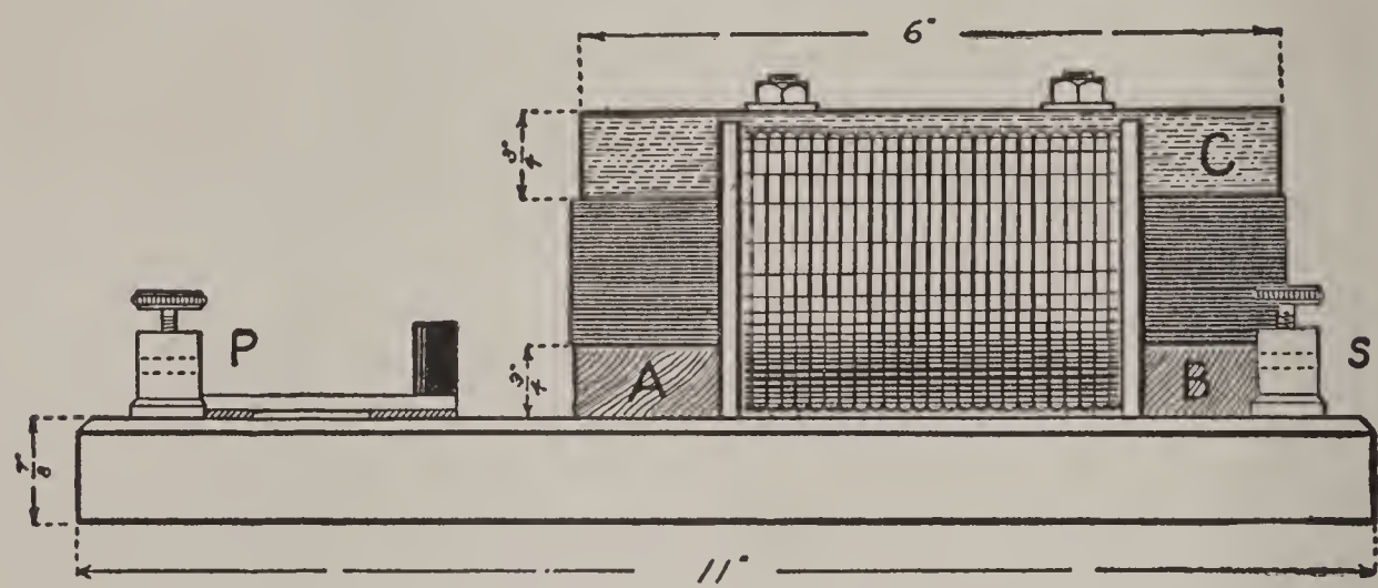
FIG. 192. — Side View of the Transformer.
