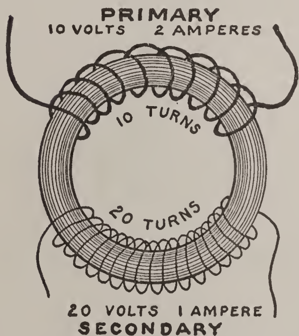
FIG. 178. — Step-Up Transformer.
