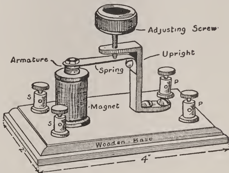
FIG. 213. — The Relay.
