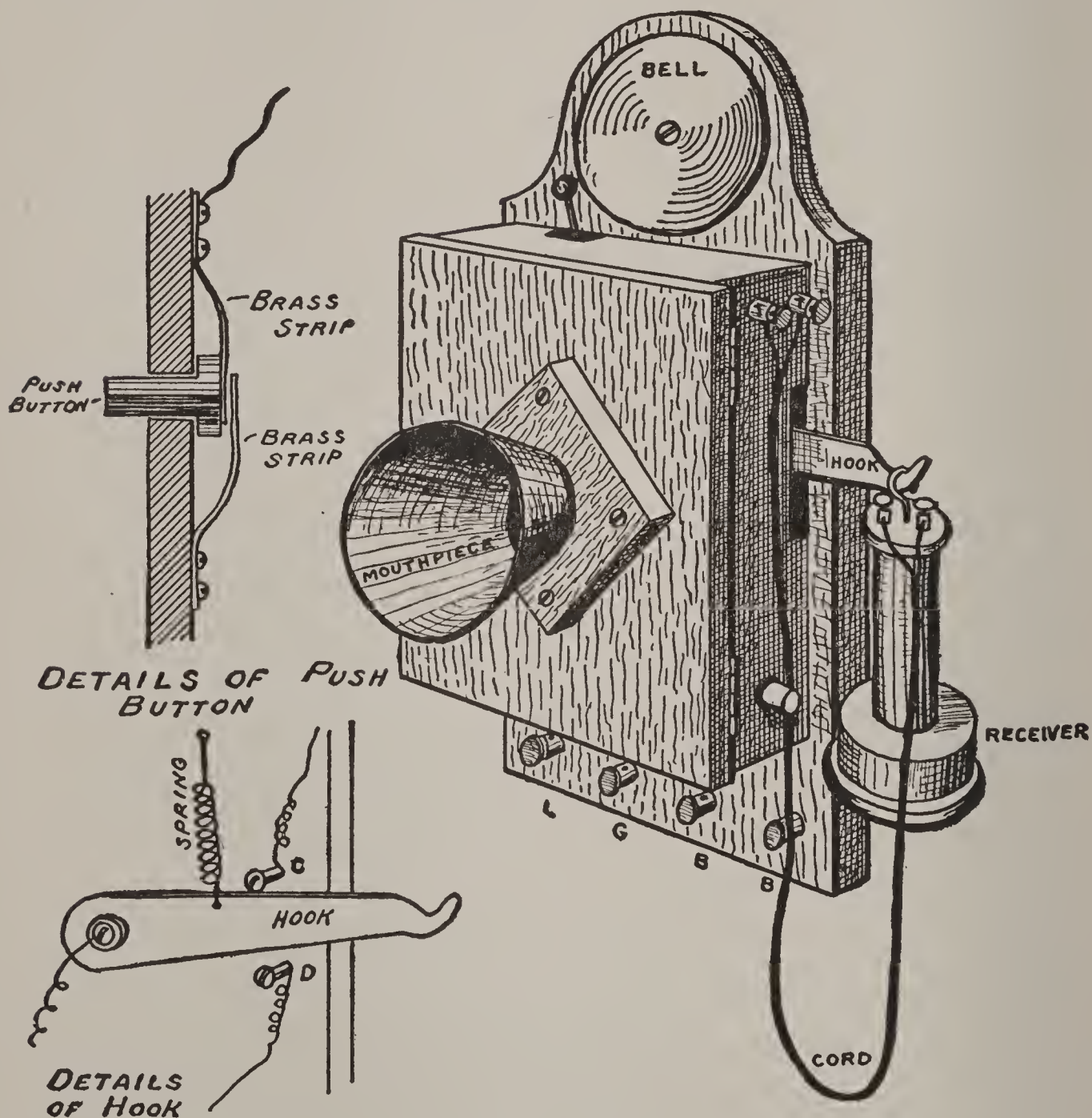
FIG. 149. — A Complete Telephone Instrument.
