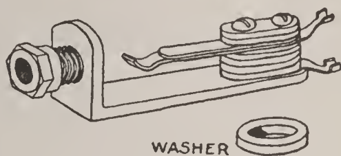
FIG. 231. — A Jack.
