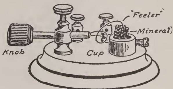
FIG. 203. — Another Form of the "Cat-Whisker" Detector.
