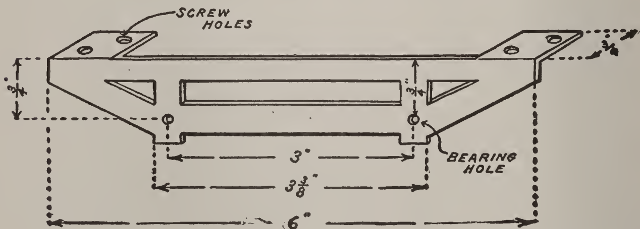
FIG. 270. — Details of the Bearing which supports the Wheel and Axle.
