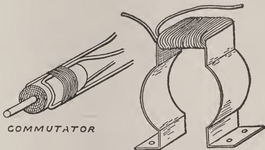
FIG. 251. — The Field and Commutator.
