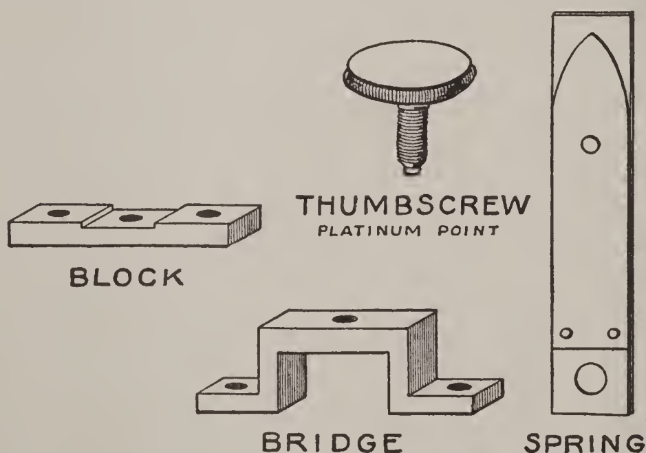
FIG. 164. — Interrupter Parts.
