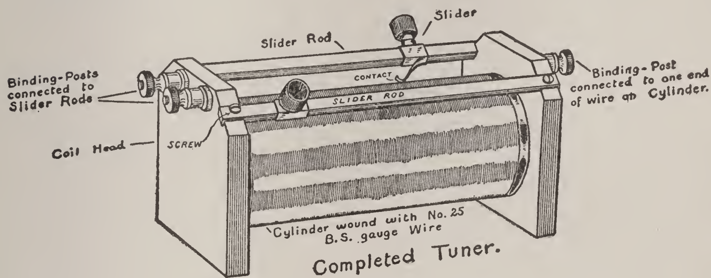
FIG. 201. — Complete Double-Slider Tuning Coil.
