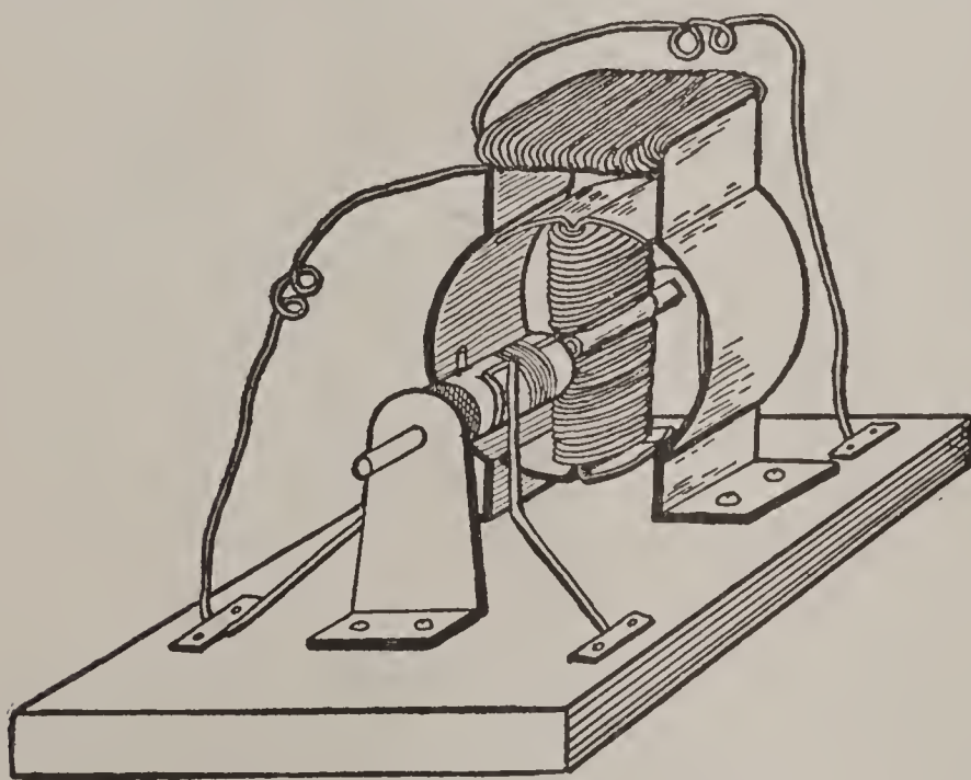
FIG. 253. — The Complete Motor.
