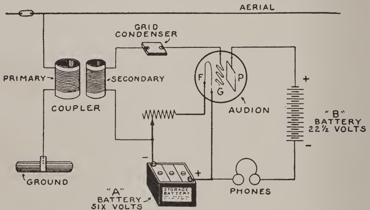
FIG. 219. — A Simple Audion Receiving Circuit.
