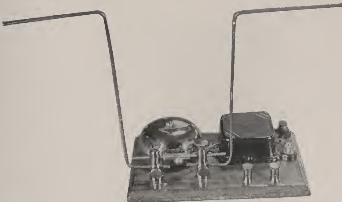
A COMPLETE COHERER OUTFIT AS DESCRIBED ON PAGE 258.
