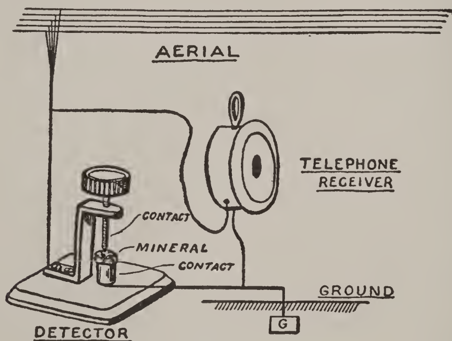
FIG. 195. — A Simple Receiving Station.
