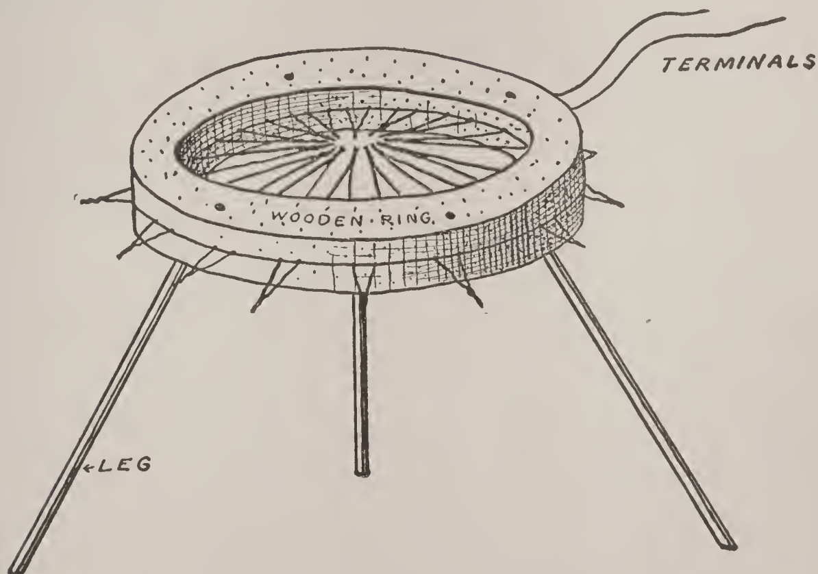
FIG. 309. — Complete Thermopile.
