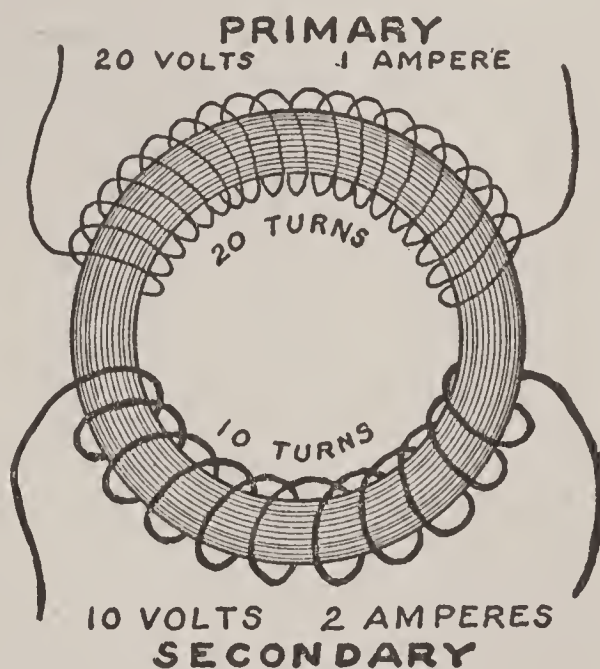
FIG. 179. — Step-Down Transformer.
