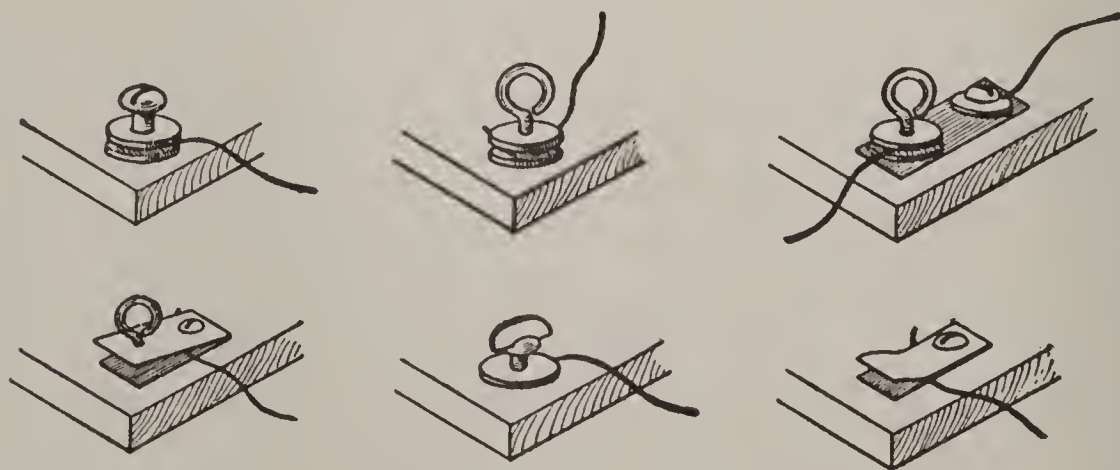
FIG. 93. — Home-made Binding-Posts.
