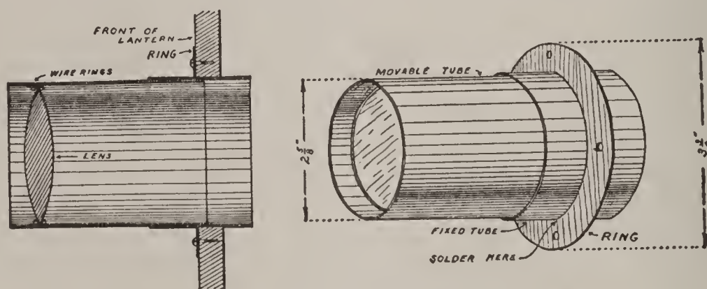
FIG. 311.—How the Lens is Arranged and Mounted.
