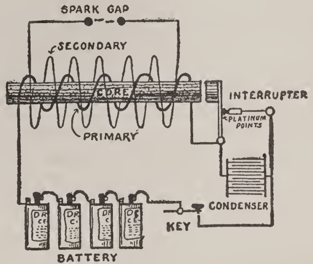
FIG. 157. — Diagram showing Essential Parts of Induction Coil.
