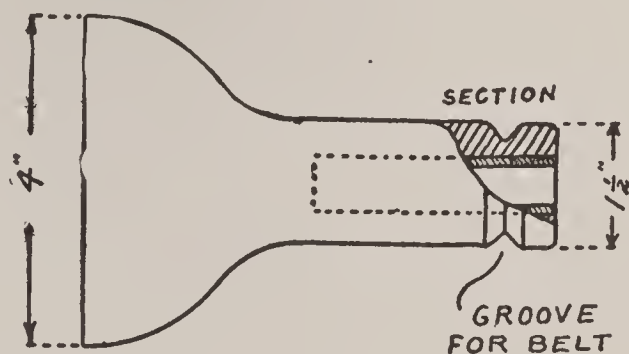
FIG. 36. — A Side View of one of the Bosses, showing the Brass Bushing used.
