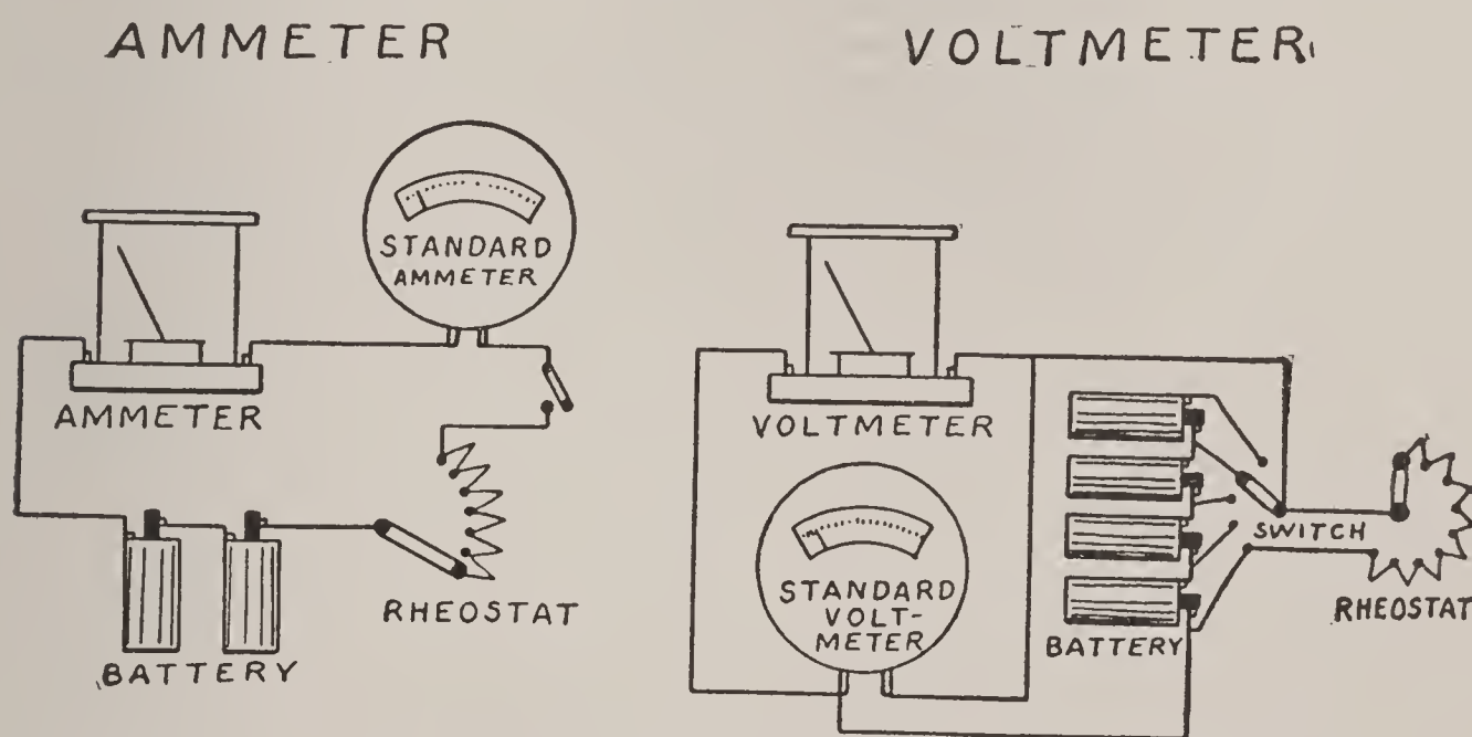
FIG. 109. — Circuits for Calibrating the Ammeter and Voltmeter.
