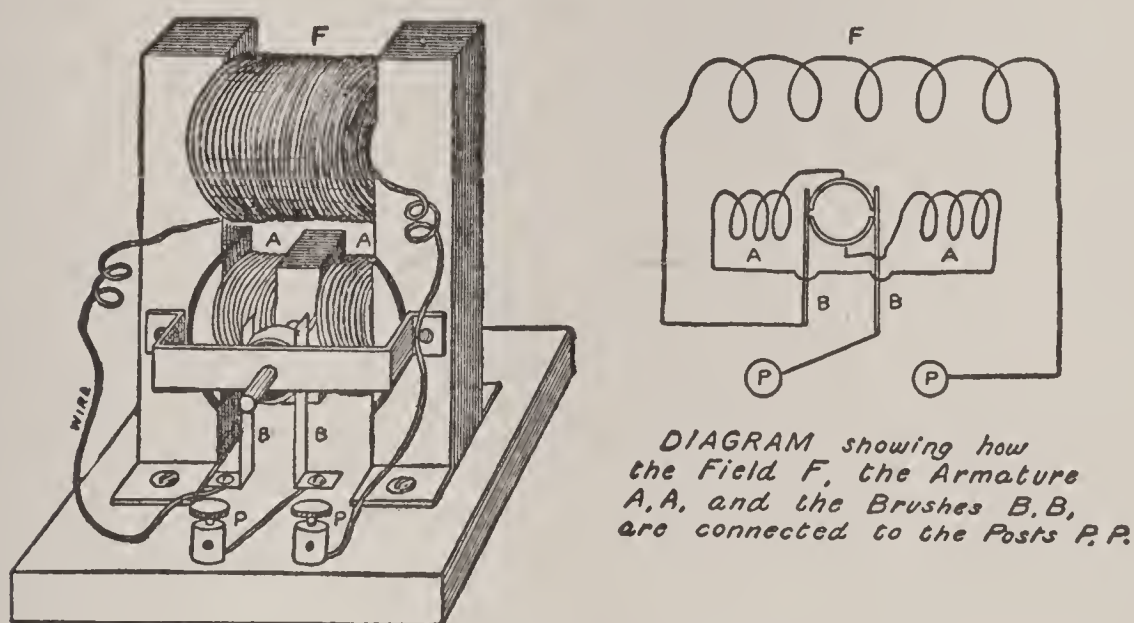
FIG. 255. — Complete Motor.
