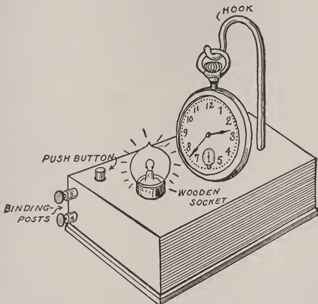
FIG. 303. — A Watch-Light.
