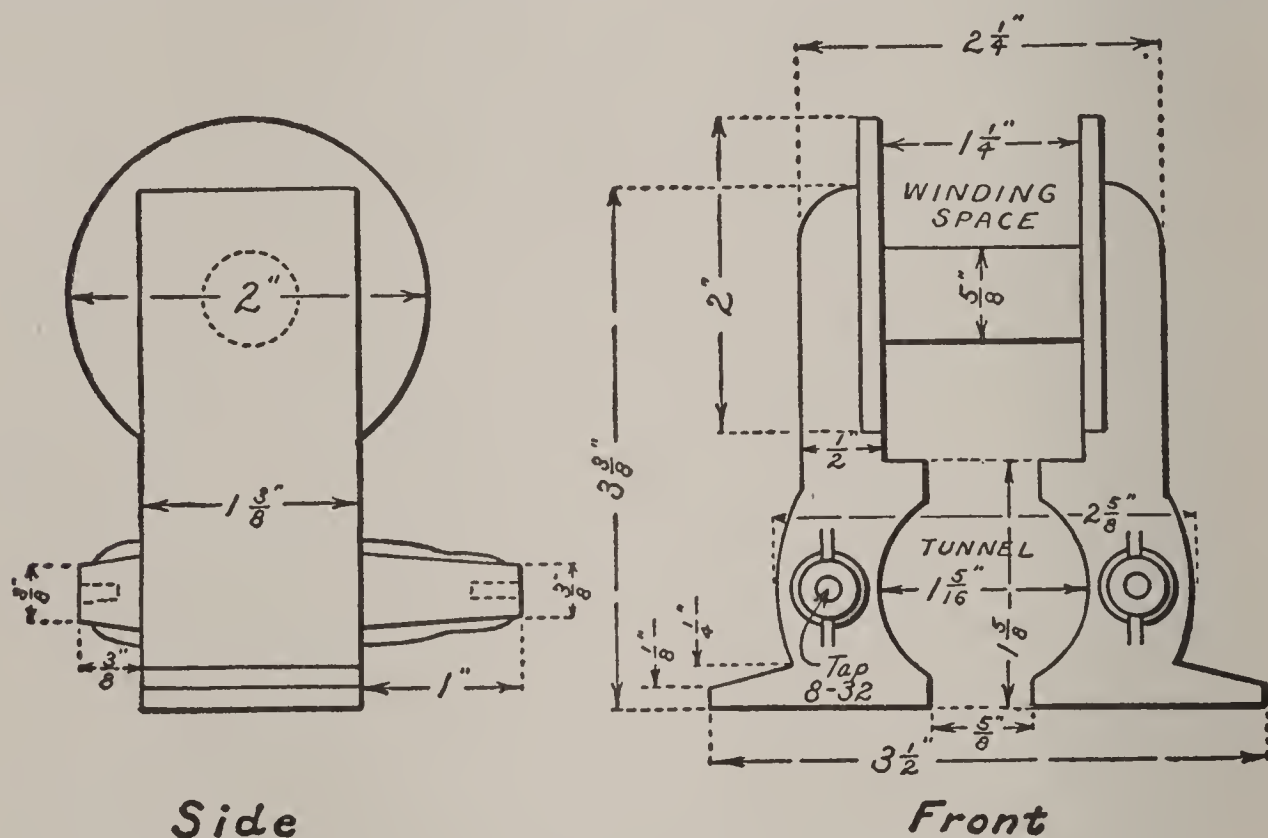
FIG. 260. — Details of the Field Casting.
