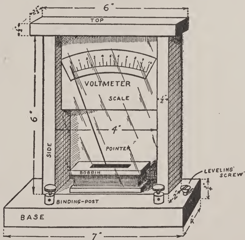
FIG. 108. — Completed Voltmeter.
