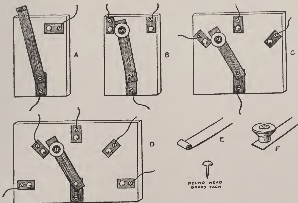
FIG. 95. — Simple Switches.
