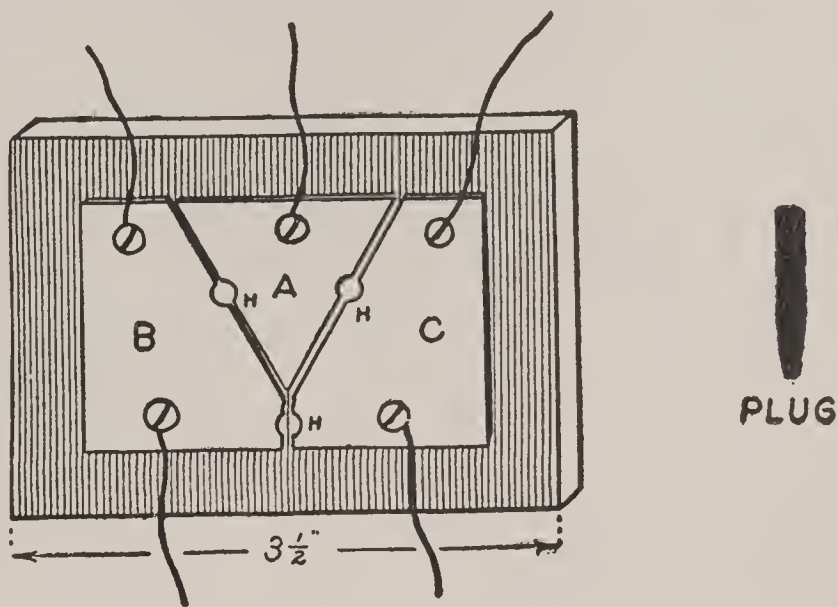
FIG. 100. — Home-made Lightning-Arrester.
