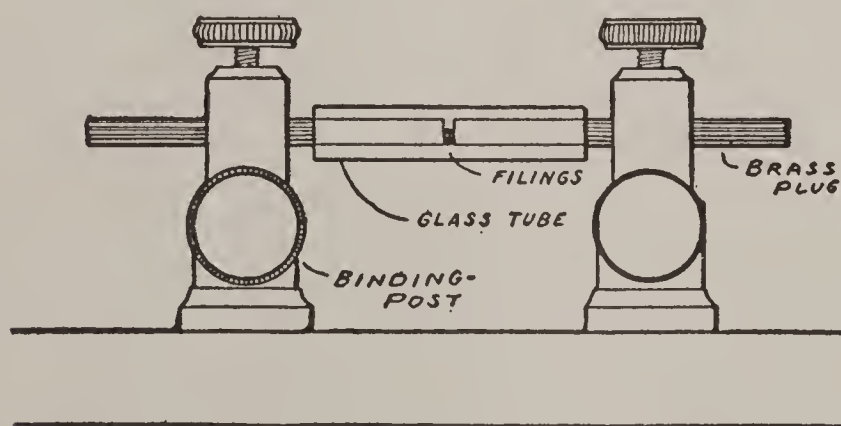
FIG. 212. — Details of the Coherer,
