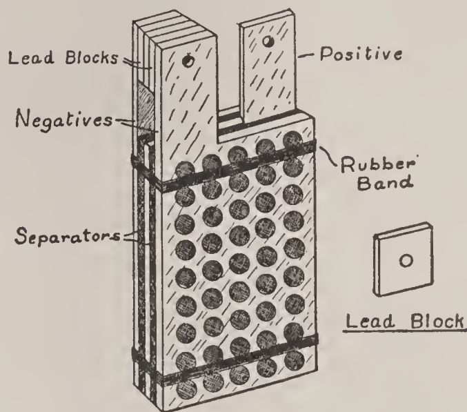
FIG. 73. — The Complete Element for a Storage Cell.
