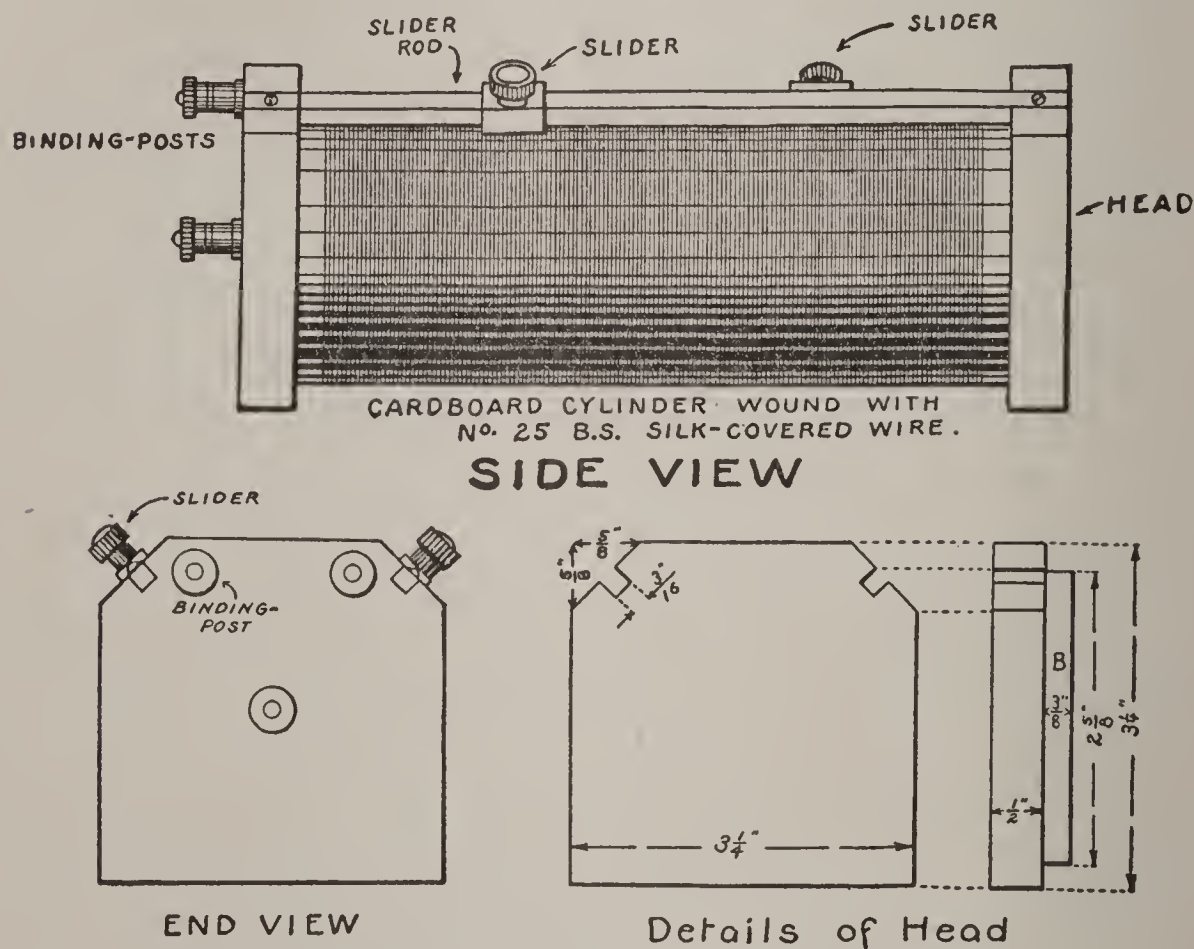
FIG. 200. — Side and End Views of the Tuning Coil.
