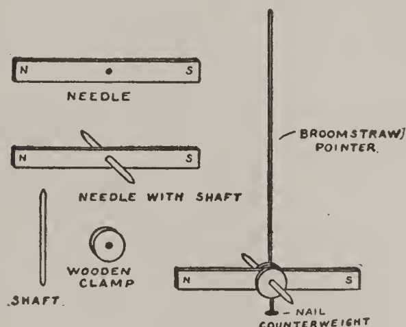
FIG. 103. — Arrangement of the Needle and Pointer.
