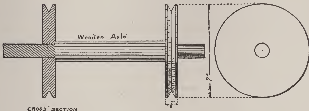
FIG. 39. — The Driving-Wheels and Axle.
