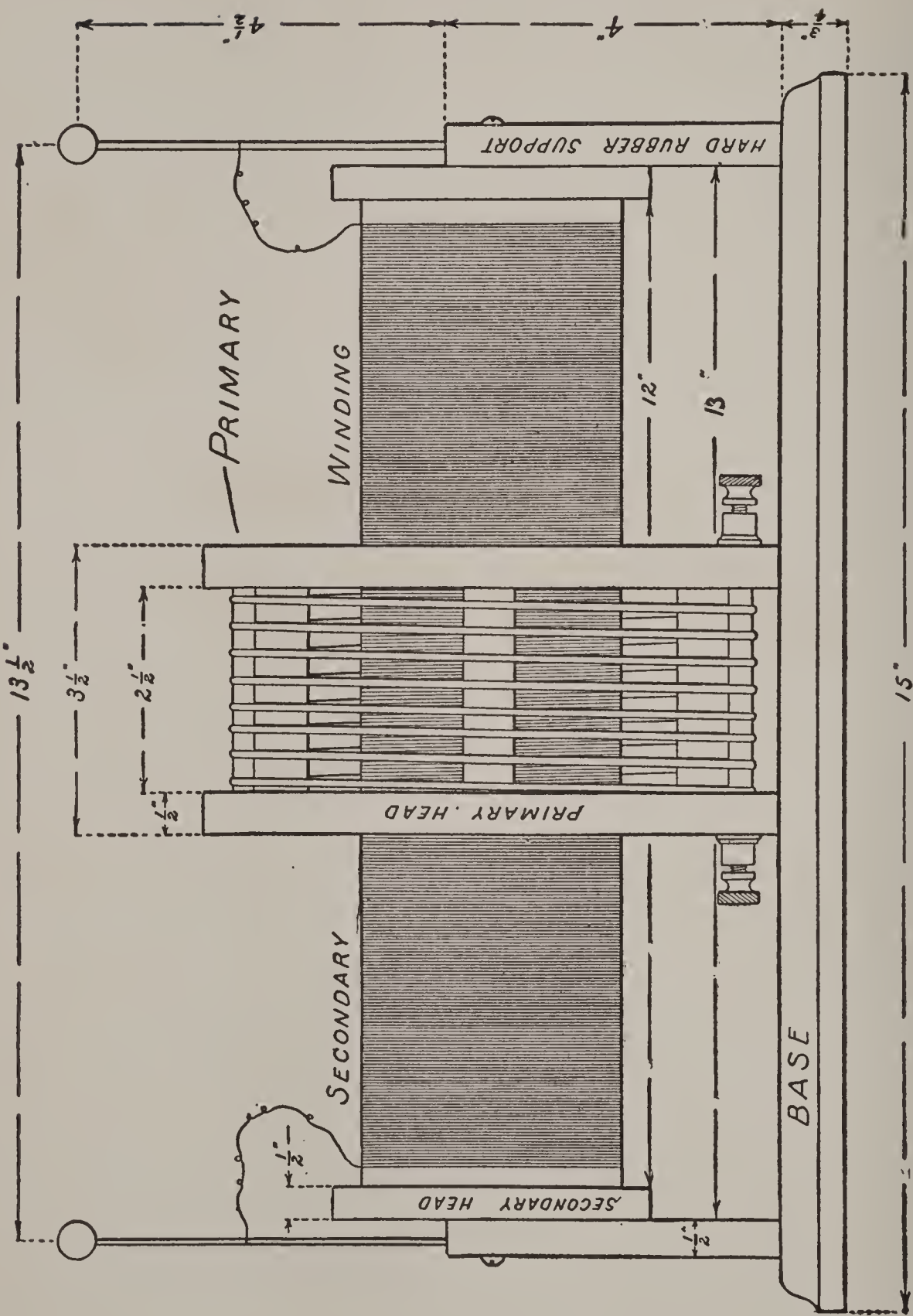
FIG. 325. — The Complete Tesla Coil.
