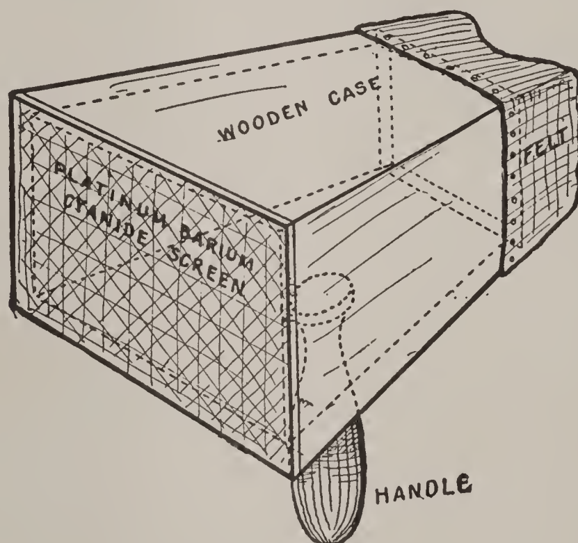
FIG. 173. — Fluoroscope.
