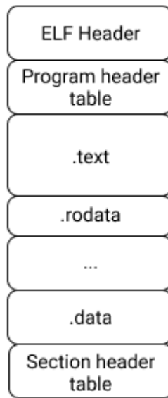
Figure 8.1: Executable and Linkable Format (ELF)
