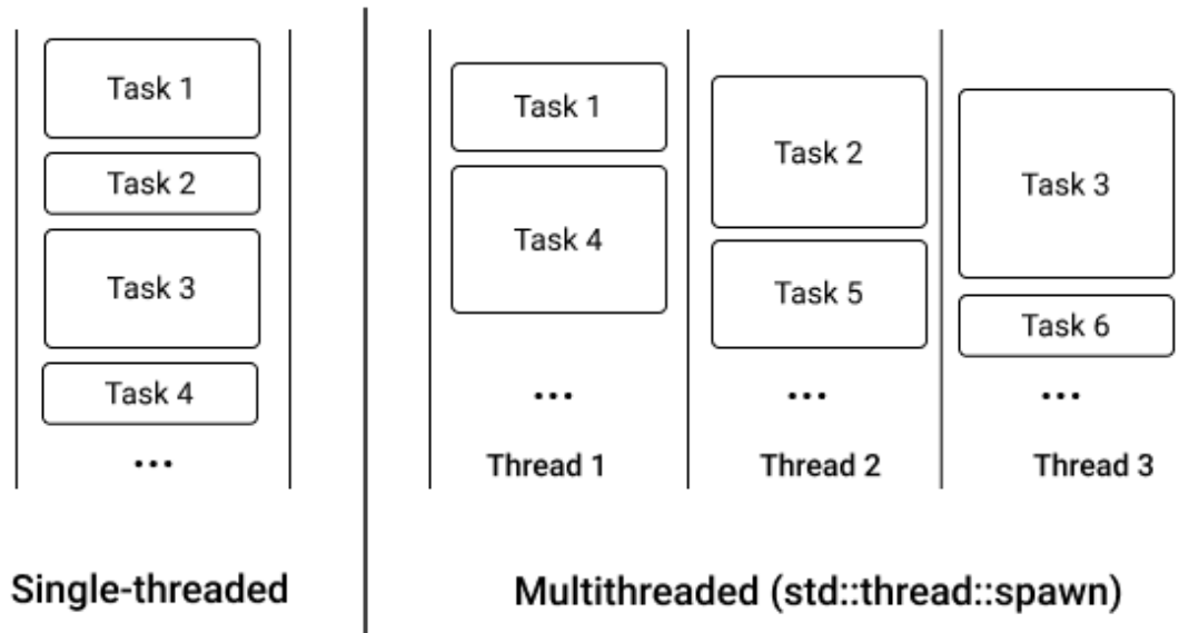
Figure 2.2: Single vs Multi threaded
