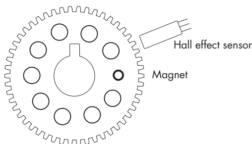
Figure 7-6: Camshaft timing sprocket
