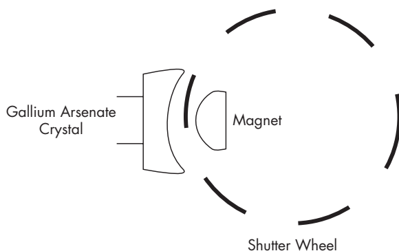
Figure 7-5: Shutter wheel diagram for Hall effect sensor
